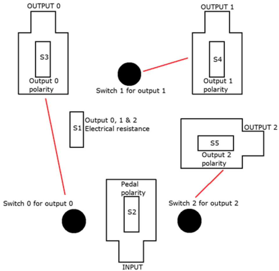
Figure 1 Bottom view
